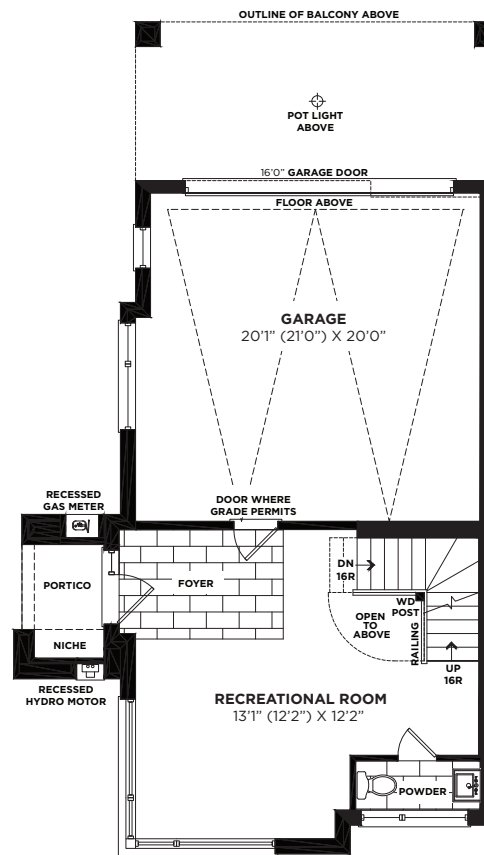
GROUND FLOOR PLAN ELEVATION 'B'
