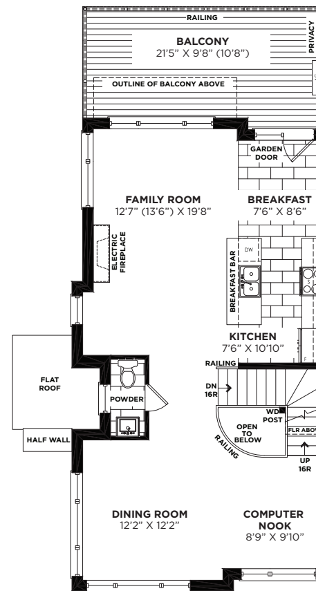
SECOND FLOOR PLAN ELEVATION 'A'
