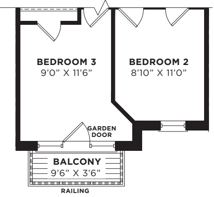
PARTIAL - THIRD FLOOR PLAN ELEVATION 'B'
