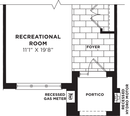
PARTIAL - GROUND FLOOR PLAN ELEVATION 'B'
