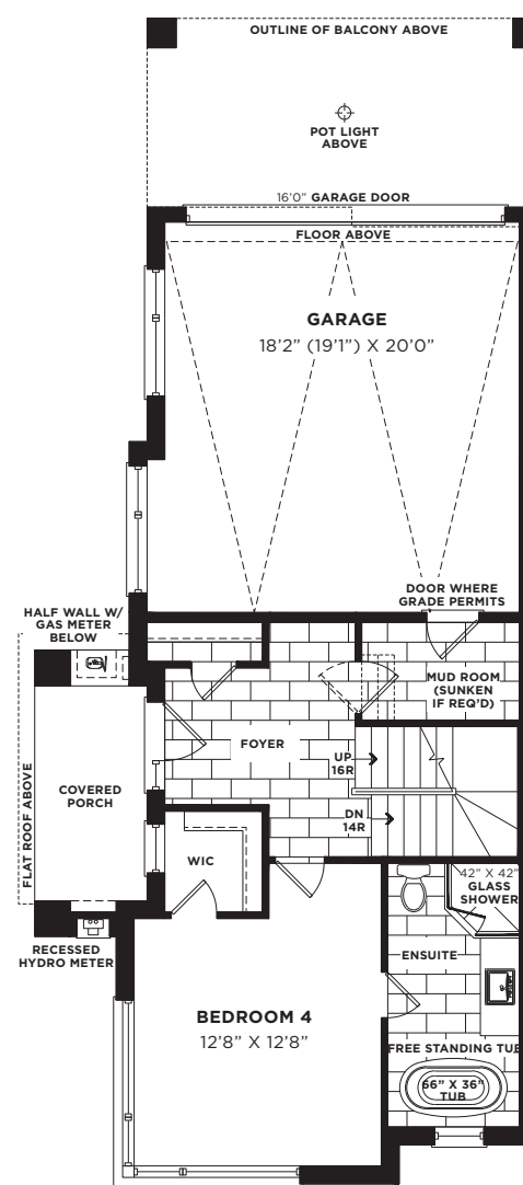
OPT. GROUND FLOOR PLAN 4 BEDROOM W/ ENSUITE ELEVATION 'A'
