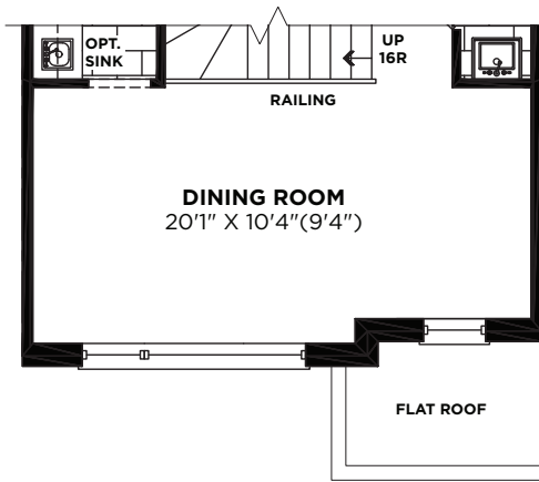
PARTIAL SECOND FLOOR PLAN ELEVATION 'B'
