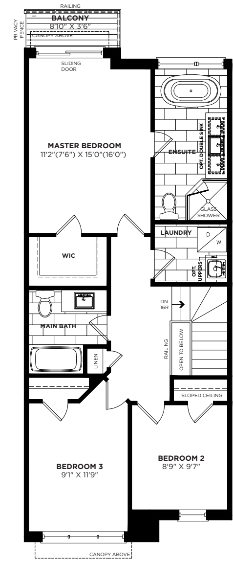
THIRD FLOOR PLAN ELEVATION 'A'
