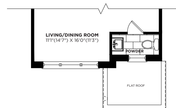
PARTIAL SECOND FLOOR PLAN ELEVATION 'B'
