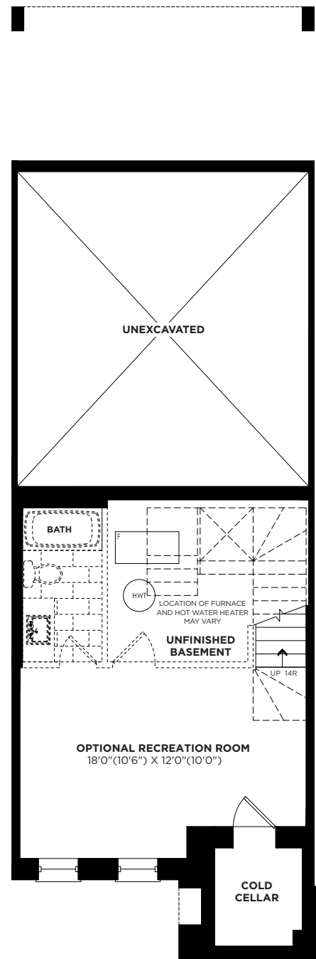
BASEMENT FLOOR PLAN ELEVATION 'A'
