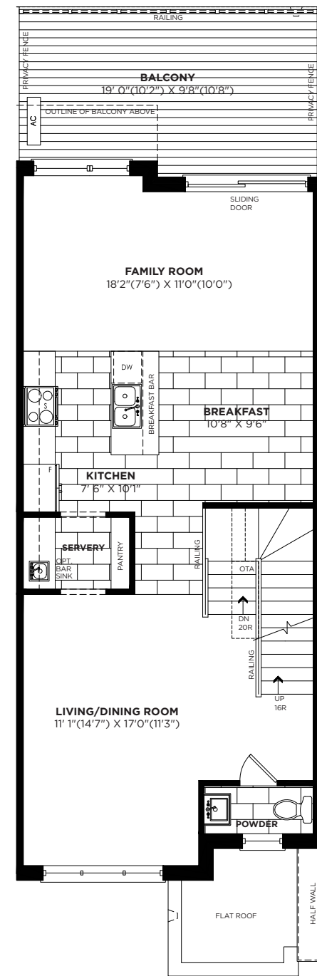
SECOND FLOOR PLAN ELEVATION 'A'
