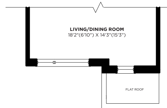
PARTIAL SECOND FLOOR PLAN ELEVATION 'B'
