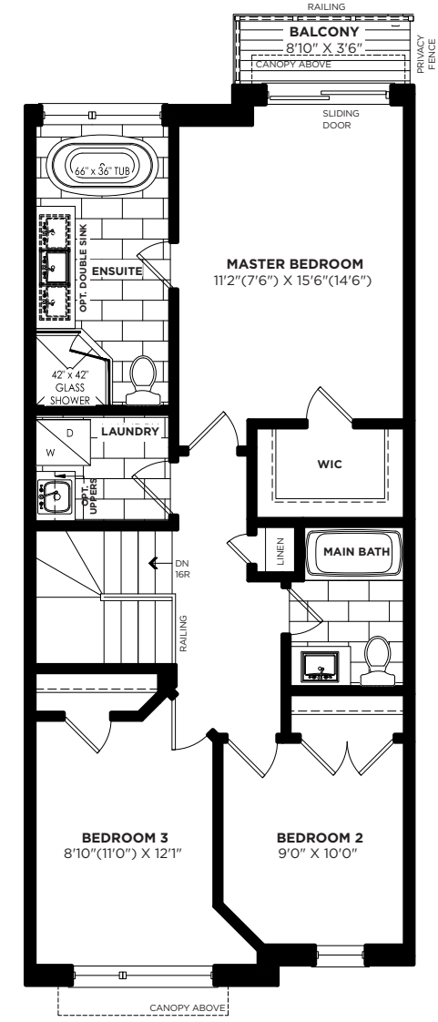
THIRD FLOOR PLAN ELEVATION 'A'
