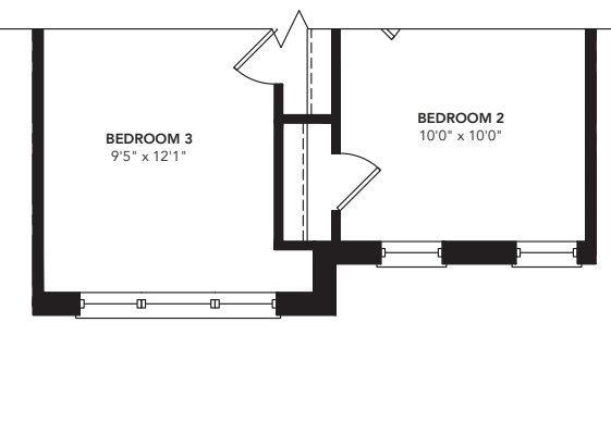
PARTIAL THIRD FLOOR PLAN ELEVATION 'B'
