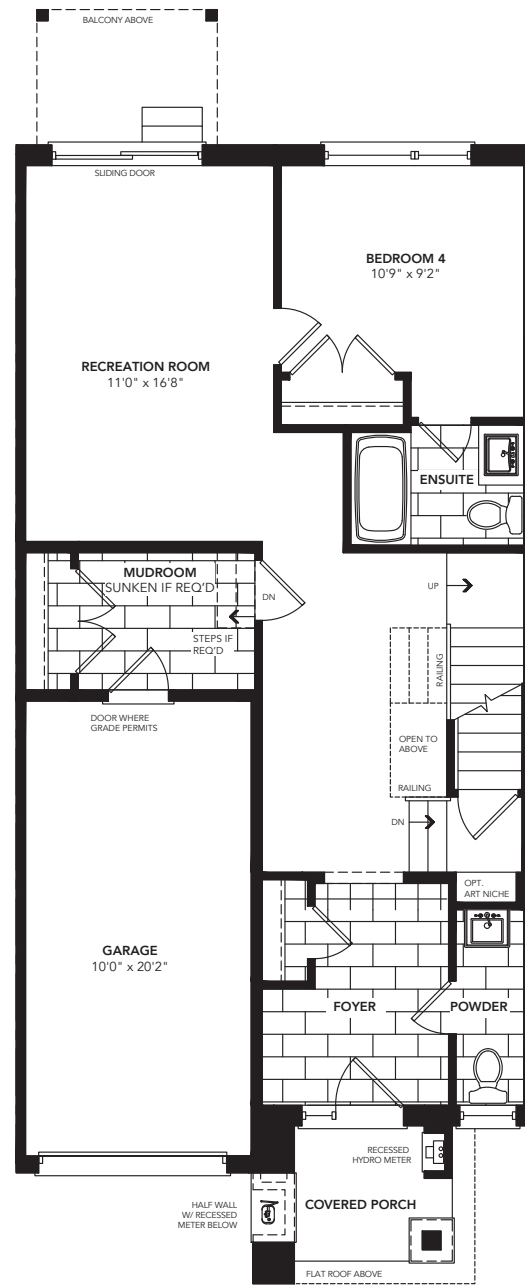
OPTIONAL GROUND FLOOR PLAN ELEVATION 'A' 4 BEDROOM WITH BATH
