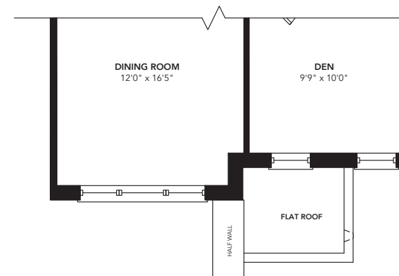
PARTIAL SECOND FLOOR PLAN ELEVATION 'B'
