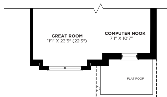
SECOND FLOOR PLAN ELEVATION 'B' (INTERIOR END)
