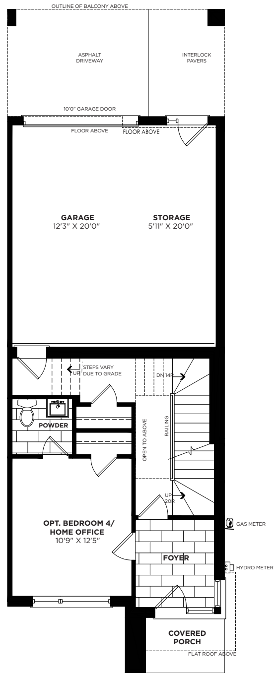
GROUND FLOOR PLAN ELEVATION 'A' (INTERIOR END)
