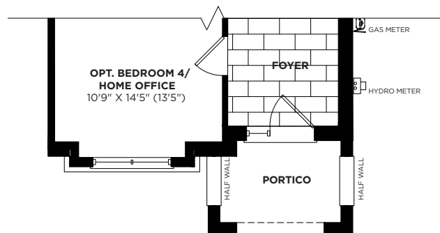
GROUND FLOOR PLAN ELEVATION 'B' (INTERIOR END)
