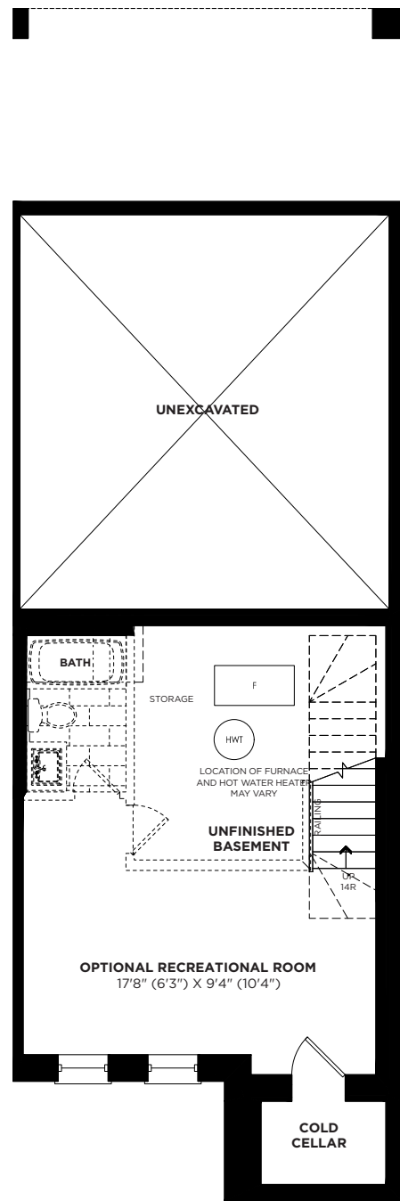
BASEMENT FLOOR PLAN ELEVATION 'A' (INTERIOR END)
