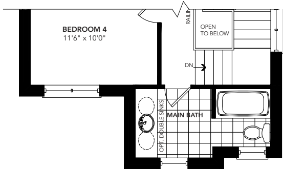
SECOND FLOOR PLAN ELEVATION 'B'
