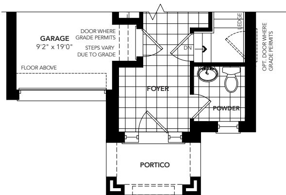
GROUND FLOOR PLAN ELEVATION 'C'
