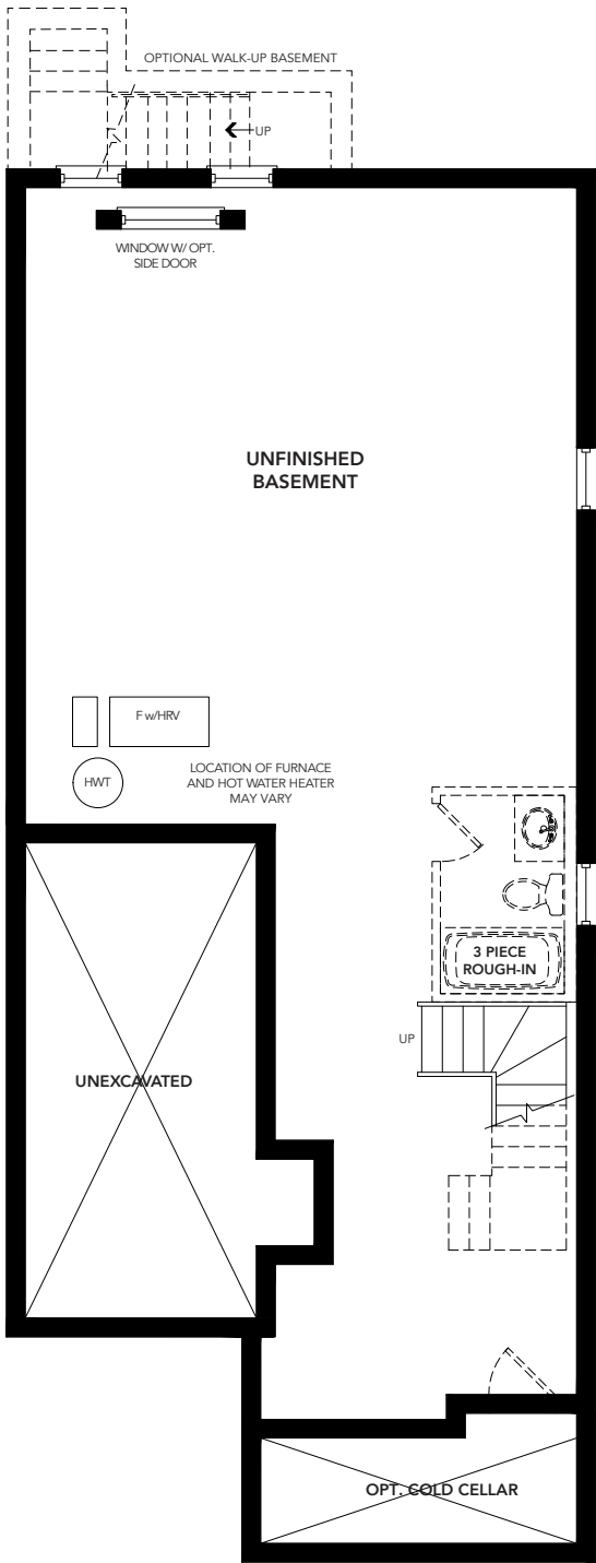
BASEMENT FLOOR PLAN ELEVATION 'A'
