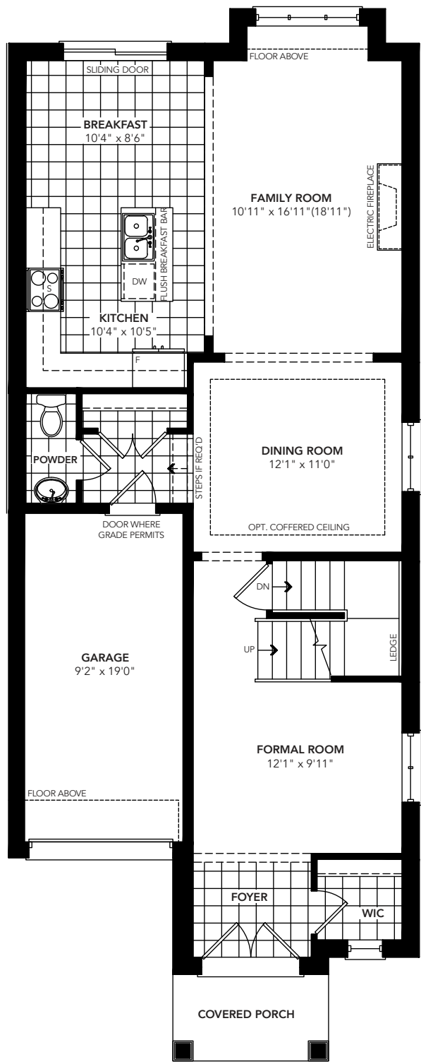
GROUND FLOOR PLAN ELEVATION 'A'
