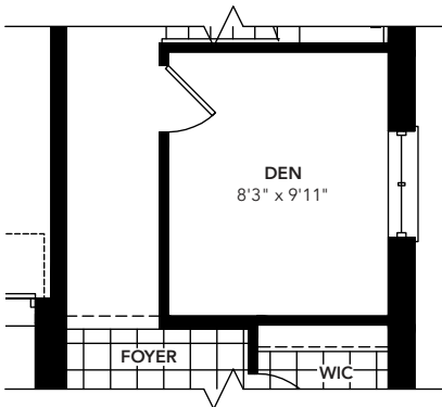
PART. OPT. GROUND FLOOR W/ DEN ELEVATION 'A', 'B' & 'C'
