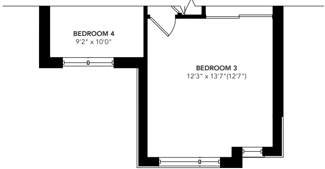
SECOND FLOOR PLAN ELEVATION 'C'
