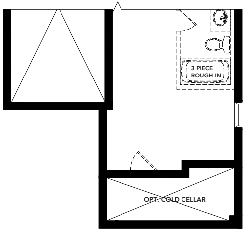
BASEMENT FLOOR PLAN ELEVATION 'B' & 'C'
